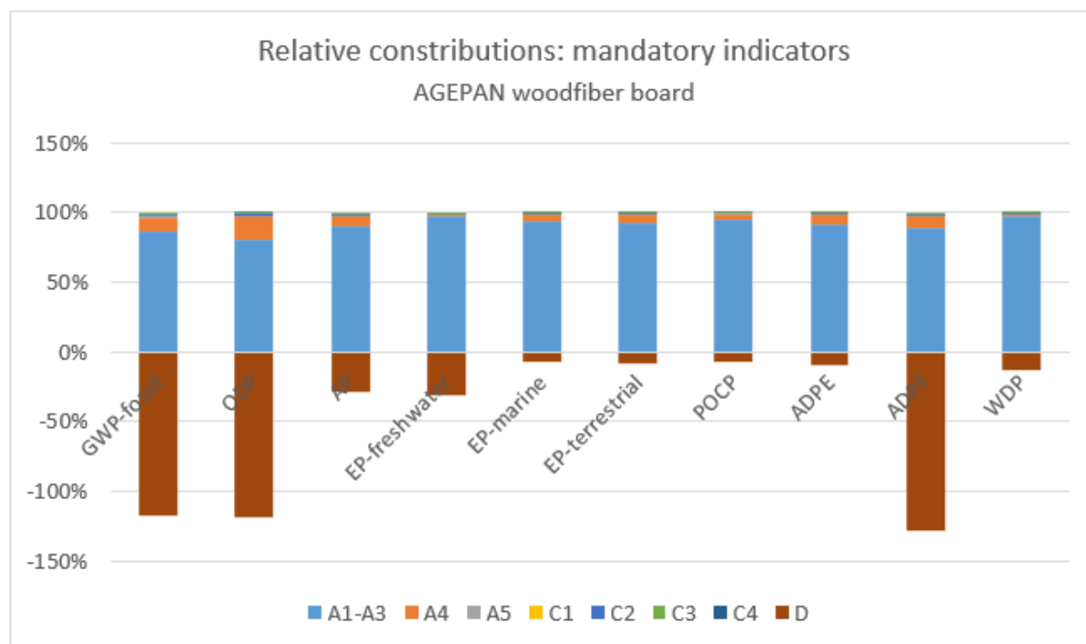
Figure 1: Environmental impacts of AGEPAN® Wood Fibreboard along its life cycle (impacts from production modules A1-C4 = 100)
